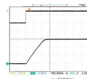
Typical Start-Up Wave Form
